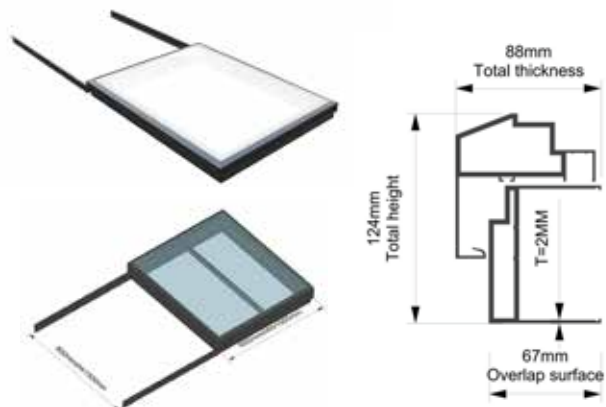
Material: 6063-T5 Aluminium profile
