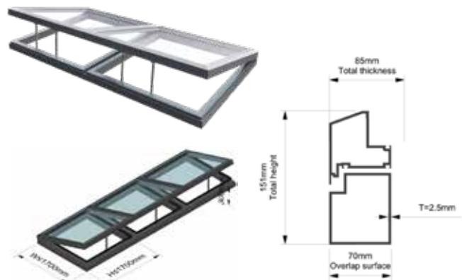
Material: 6063-T5 Aluminium profile
