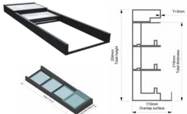
Material: 6063-T5 Aluminium profile
