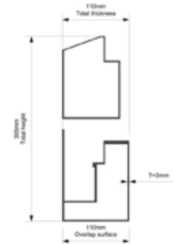
Material: 6063-T5 Aluminium profile
