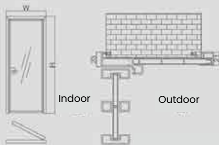
Italian-style patchwork double-sided hinged door assembly diagram
