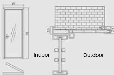
Italian-style double-sided swing door assembly diagram
