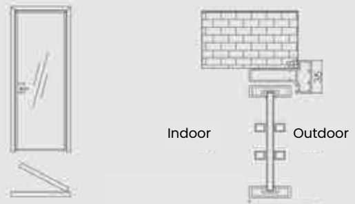
Italian-style light and shadow single-pack hinged door assembly diagram
