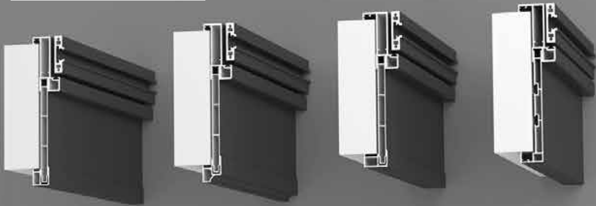
Ultra-narrow flat double pack
