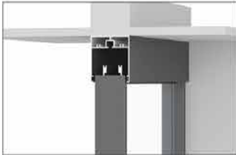
Monorail push-pull track Track dimensions: 47.8*87.8
