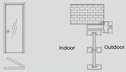
Italian-style patchwork single-pack hinged door assembly diagram
