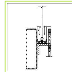
Fascia Mount
