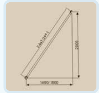
DIAGONAL BRACE DB-140200, 1.4x2.0m, 2.8kg(6.2lbs) DB-140200, 1.8x2.0m, 3.0kg(6.6lbs) DB-250150, 2.5x1.5m, 3.2kg(7.1lbs)
