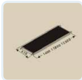
PLATFORM P-140, 1.4m, 10.9 kg (24.0lbs) P-180, 1.8m, 13.5kg (29.8lbs) P-250, 1.8m, 18.7kg (41.2lbs)
