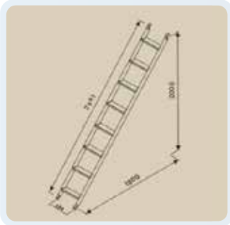
STAIR LADDER 1.8m x 2.0m SL-180200, 8.9kg(19.6lbs)
