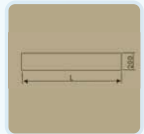
TOE BOARD TB-078 L = 570 mm, 0.88kg (1.9lbs) TB-140 L = 1180 mm, 1.80kg (4.0lbs) TB-140 L = 1280 mm, 2.00 kg (4.4lbs) TB-180 L = 1667 mm, 2.60kg (5.7lbs) TB-250 L = 2380 mm, 5.40 kg (12.0lbs)
