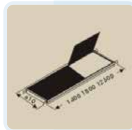
TRAPDOOR PLATFORM TP-140, 1.4m, 11.1kg (24.5lbs) TP-180, 1.8m, 13.9kg (30.6lbs) TP-250, 2.5m, 19.1kg (42.1lbs)
