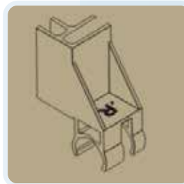
TOE BOARD HOLDER (RIGHT) TH-01R, 0.34kg(0.75lbs)
